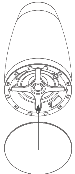
FIGURE 21: GRILLE INSTALLATION
