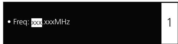
Select frequency
